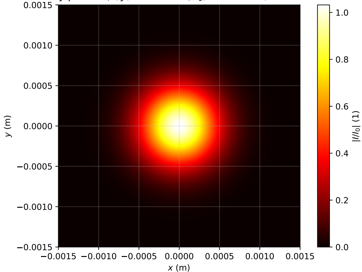
Intensity profile I(x, y, z = 0.318m)/I_0 , P_{in}=0.6P_{cr} , artificial time
